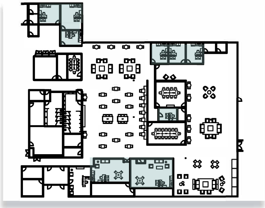
FLOOR PLANS
