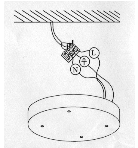
Electrical Connection
