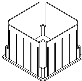
10816 - ONE WAY INTERNAL POST CONNECTOR (X6)
