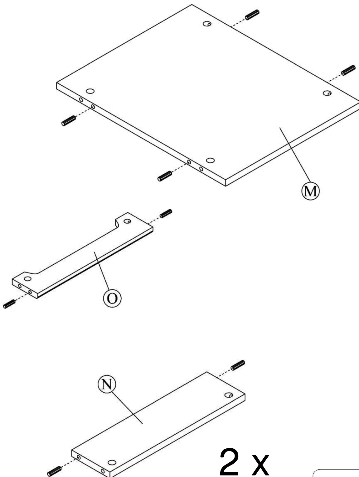
Wood Dowel 8 x 30mm
