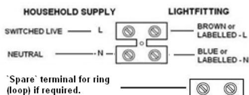
Details of terminal wiring.
