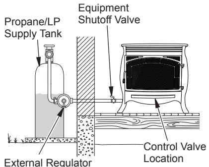
Figure 14 - Checking Gas Joints for Propane/LP Gas
