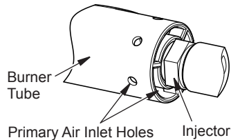
Figure 30 - Burner and Injector Holder
