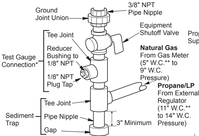
Figure 11 - Gas Connection
